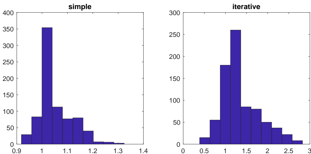
Figure 10: Distribution of \lambda for the US
